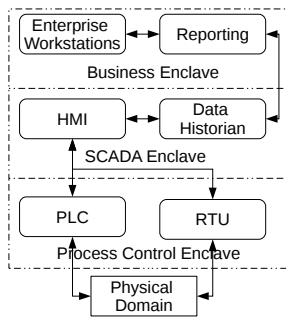
Figure 1: high-level view of an ICS network.
